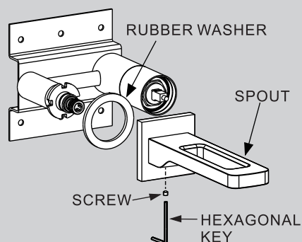
FIG. 1 INSTALLATION OF SPOUT
