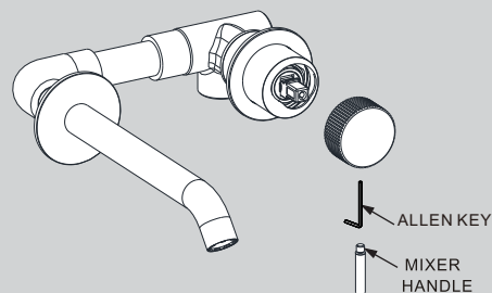
FIG. 2 INSTALLATION OF HANDLES
