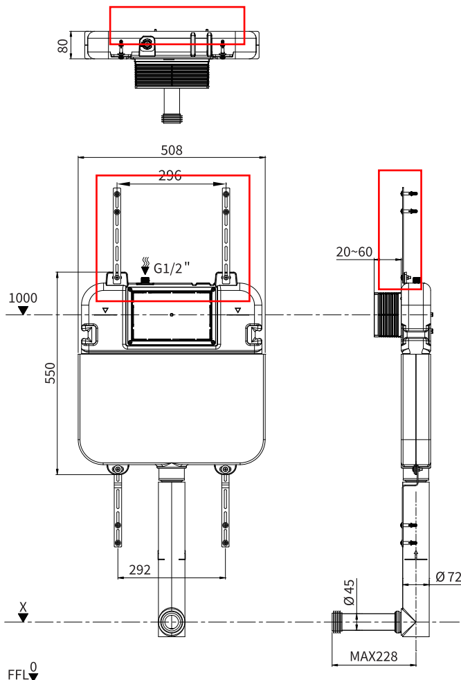
General dimension and water supply drawing. Water supply to cistern. (water supply should be connection to angle valve inside cistern)
