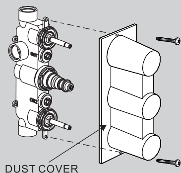
FIG. 1 FITTING PLASTIC DUST COVER
