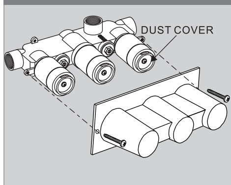
FIG. 1 FITTING PLASTIC DUST COVER
