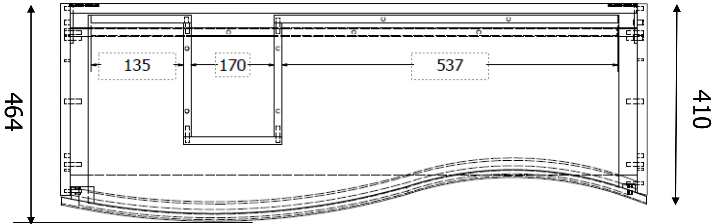
Plan View
