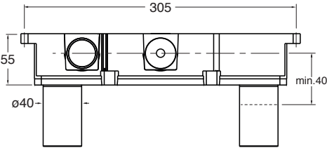
NOTE: ALL DIMENSIONS IN MILLIMETERS
