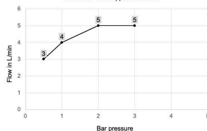
Flow rates with supplied restrictor
