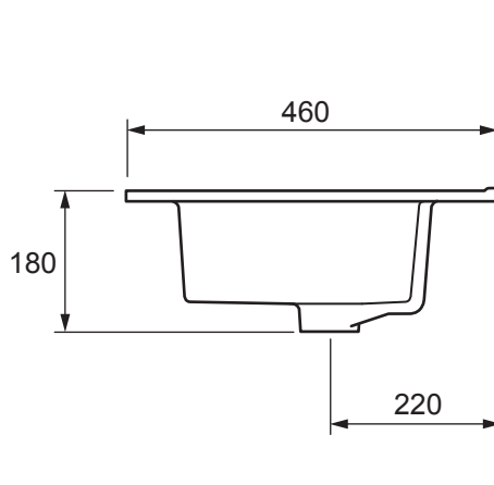
Side view on arrow
