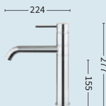
Design Single Lever Kitchen Mixer DE716DC
