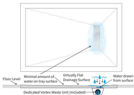
Linear Waste Shower Tray
