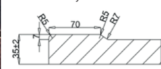
Tray Profile
