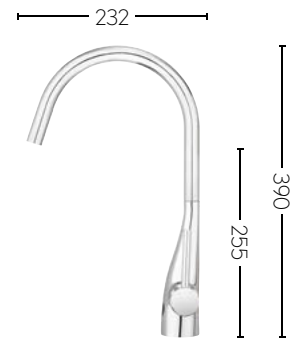
Side lever sensor kitchen mixer COX714DC £319.00 see page 373.
