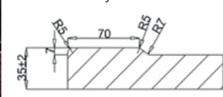
Tray Profile
